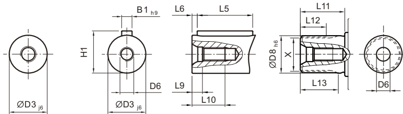
Shaft Option S1
